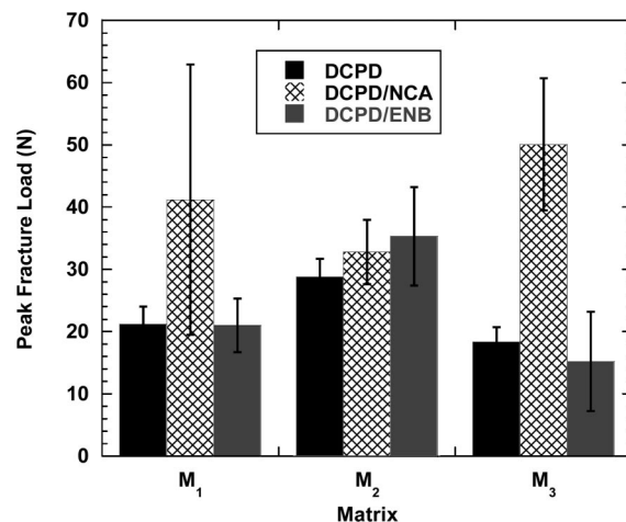
Figure 10. Average peak fracture loads of M_1 , M_2 , and M_3 samples healed with DCPD, DCPD/NCA, and DCPD/ENB. Each column is an average of data for 3–4 samples, and the error bars represent one standard deviation.
