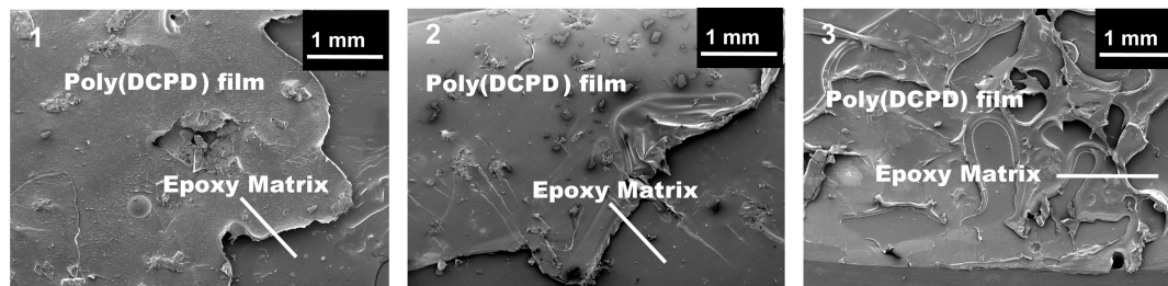
Figure 7. Scanning electron microscopy (SEM) images of representative fracture planes for self-activated epoxy ( M_1 ) samples containing 1.5 wt % as-received catalyst. Monomer (10 \mu\text{L} ) was injected into the crack plane, and the samples were left to heal for 24 h before testing. A poly(DCPD) film is observed on the surface of the epoxy matrix, which is still visible underneath. The number labels on the images correspond to the catalyst used in the matrix.
