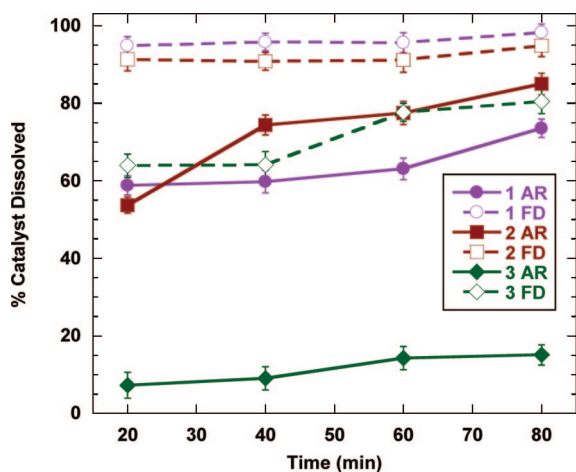
Figure 3. Comparison of dissolution rates in cyclohexane. AR designates as-received, and FD designates freeze-dried. Cyclohexane is used as a nonreactive mimic for DCPD.
